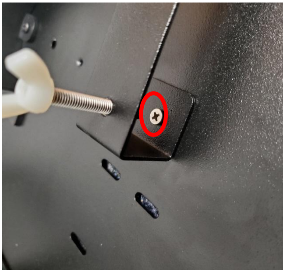
Figure 9 Splice Tray Bracket mounted by lower screw which is threaded through panel.
