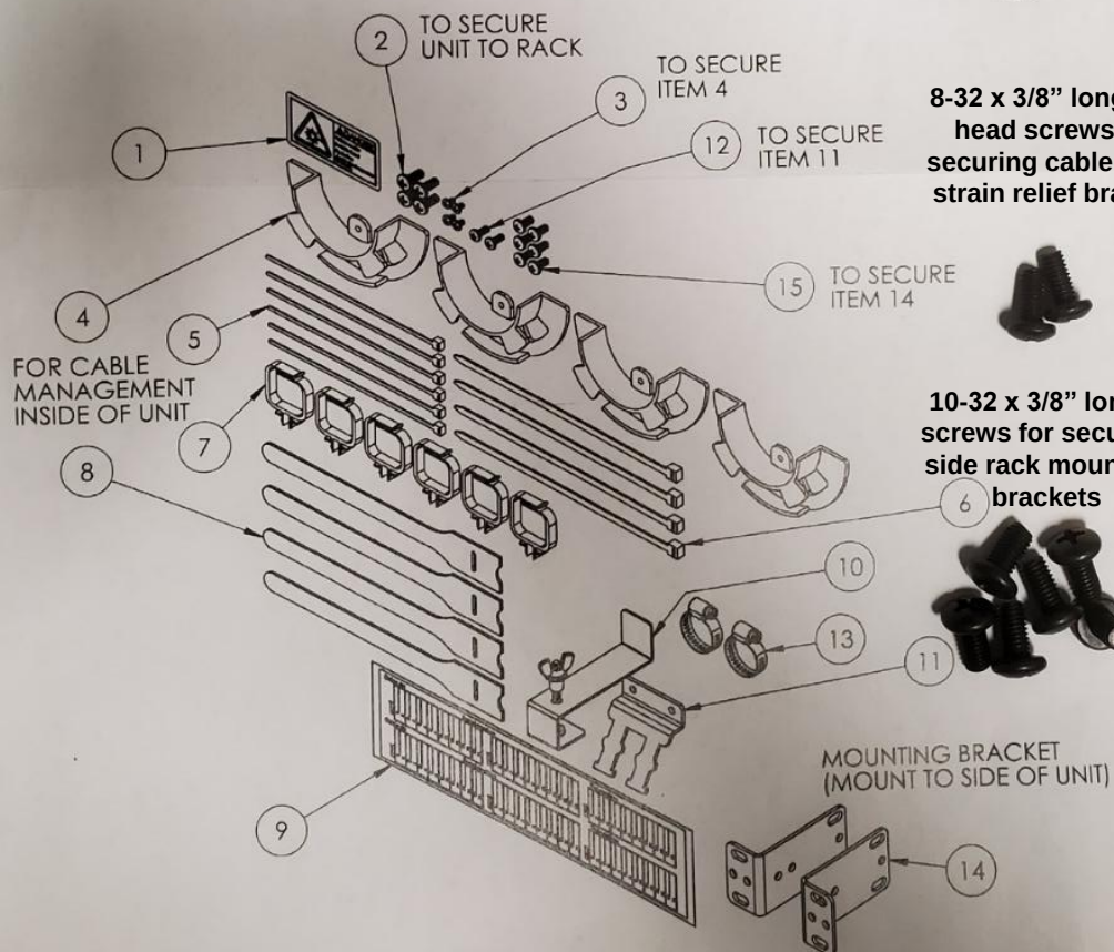
Figure 2: Sheet that comes with rack unit and description of screws provided.
