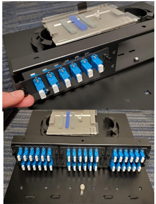
Figure 11: Adapter panels (sold separately) secured front of insert by pins.
