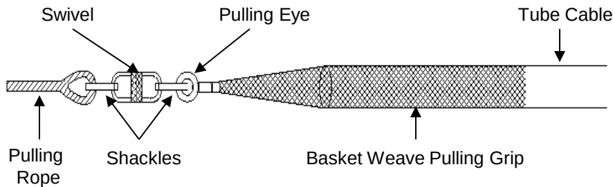
Figure 18 Standard Pulling Grip Attachment Method
