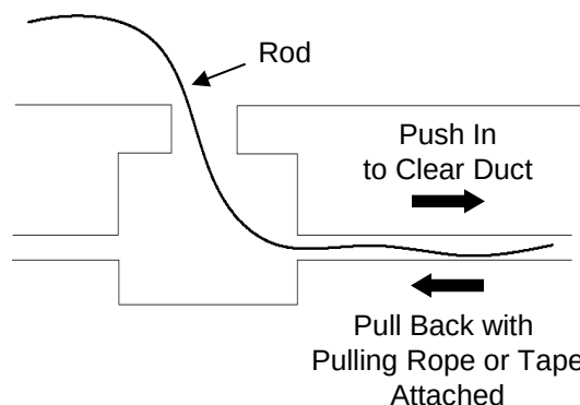
Figure 14 Rodding with a Steel or Plastic Rod
