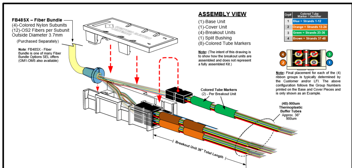
48 Fiber Breakout Kit fully assembled except for the cover unit
