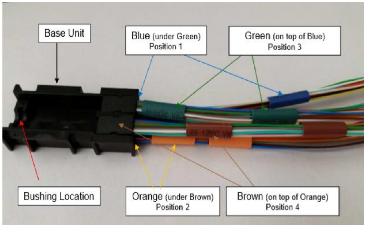
Figure 11 48 fiber breakout kit organization in Base Unit.
