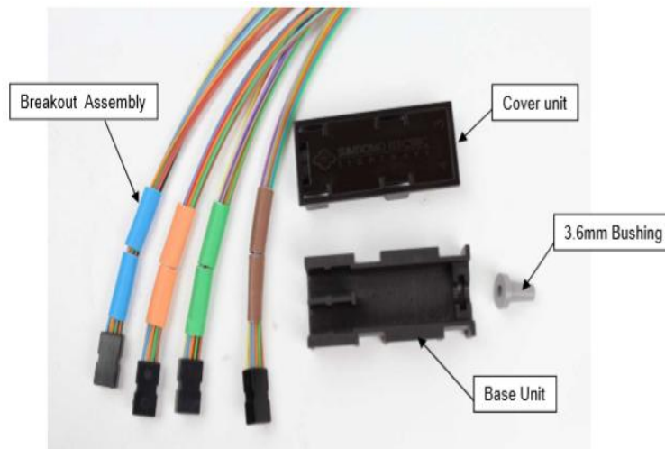
Figure 1 48 fiber bundle 900 \mu m termination kit components
