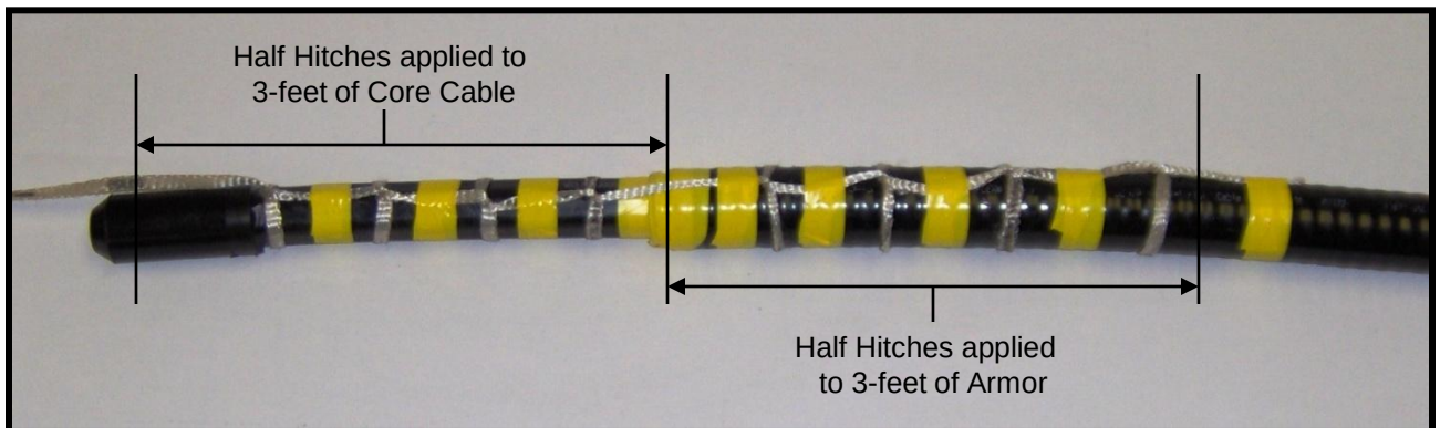
Figure 14 Pulling Tape or Rope Half-Hitched to Armor and Core Cable Equally
