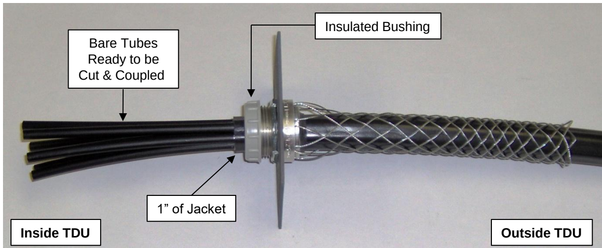
Figure 4 Dust-Tight Kellems Grip Installed and Tube Cable Ready for Coupling
