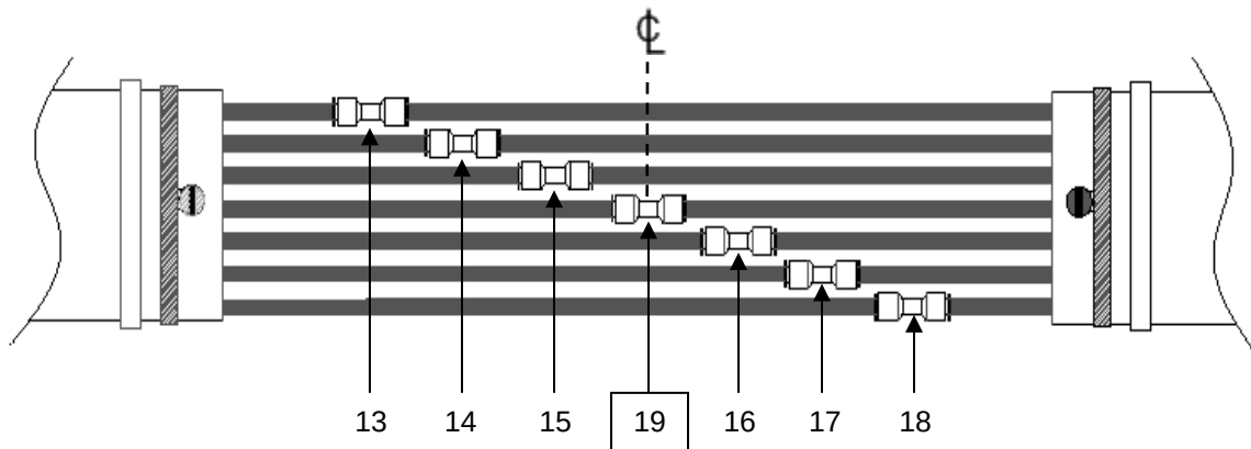
Figure 11 Couple Tube 19 in Center of Strip Length Dimension
