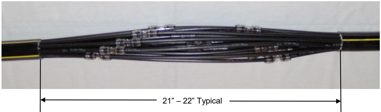
Figure 24 “Unique” Stagger Arrangement for 19-Tube Cable Example
