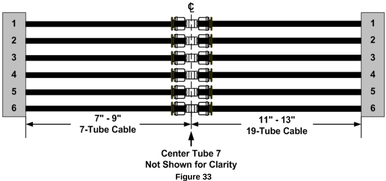
All-in-a-Row Tube Coupling Arrangement (19-Tube Cable Arrangement Similar)
