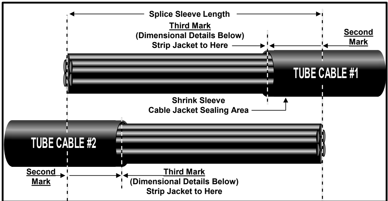
Figure 3 Stripping Tube Cables to Proper Length
