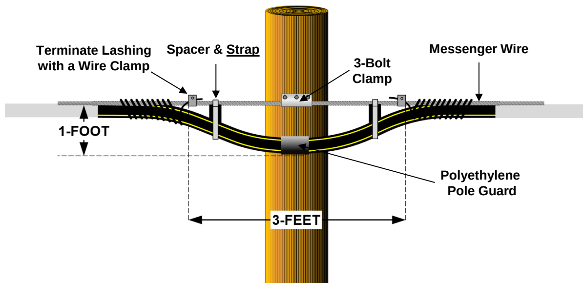
Figure 26 Tube Cable Aerial Installations Around Poles
