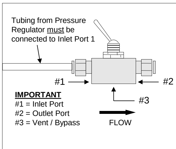
Figure 4 Bypass Switch
