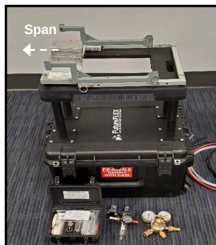
Figure 7 Blowing Head Facing Left. The BH should always face the direction of the blow.
