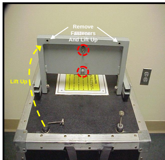
Figure 50b Payoff Stand Shelf shown Lifted for Access to the Blowing Head Fasteners
