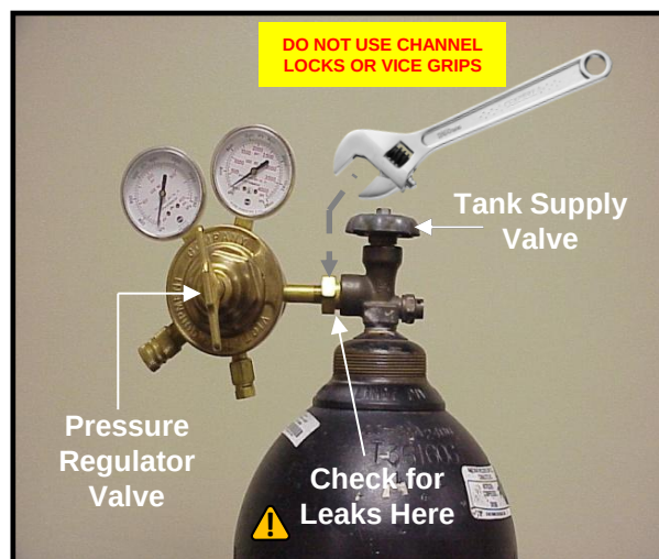
Figure 9 Pressure Regulator Connected to Gas Tank
