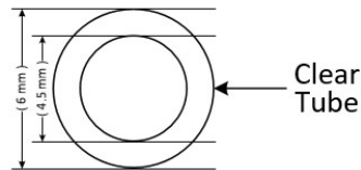
Single Tube Non-Flame Retardant P/N: TC01T6M
