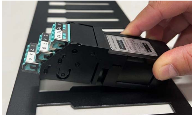
5.2 Insert the cassette from the back of the slide chassis groove.
