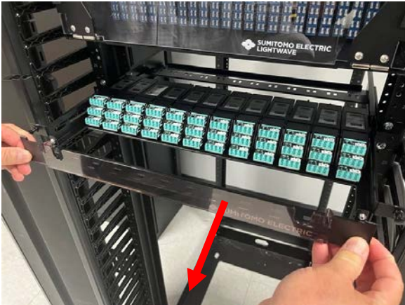
5.1 Hold both the left and right latch (black color) and pull the slide chassis to the front.
