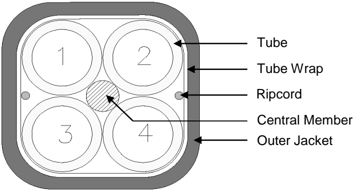
Cross Section 4-Tube TC04TP2 Drawing Not to Scale
