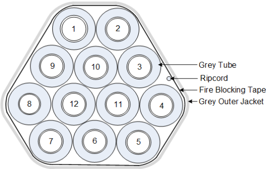
12-Tube Plenum Rated TC12TP2
