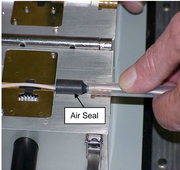
Figure 10 Open Blowing Head and Carefully Remove Fiber Bundle Air Seal
