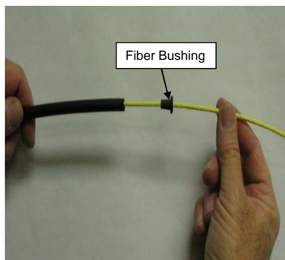
Figure 7 Install Fiber Bushing to Seal End of Tube
