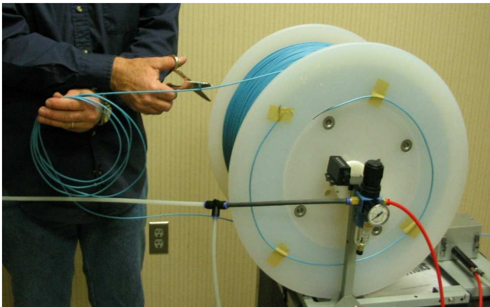
Figure 9 Fiber Bundle Still in Blowing Head (Protected) Termination Length Removed from Reel Cut Fiber Bundle from Reel
