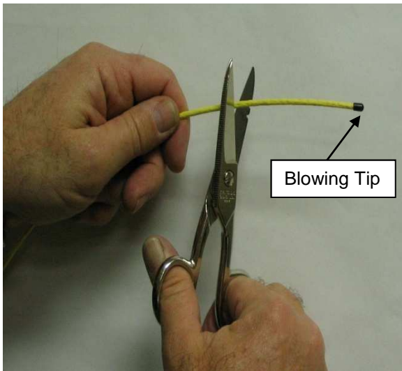
Figure 8 Do Not Remove Blowing Tip Cut 2"-3" Off End of Fiber Bundle
