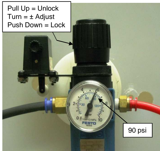
Figure 4 Set Initial Air Motor Pressure at 90 psi
