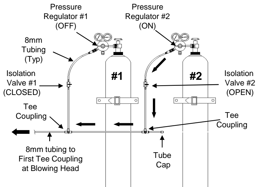
Figure 13 Dual Tank Operation; Tank #2 ON
