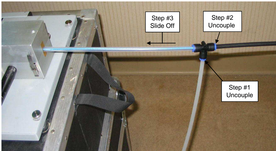
Figure 11 Step #1 = Uncouple Supply Tubing from Branch Leg of Second Tee Coupling Step #2 = Uncouple Second Tee Coupling and Clear Tube from Tube Span Step #3 = Slide Second Tee Coupling and Clear Tube off Cut End of Fiber Bundle
