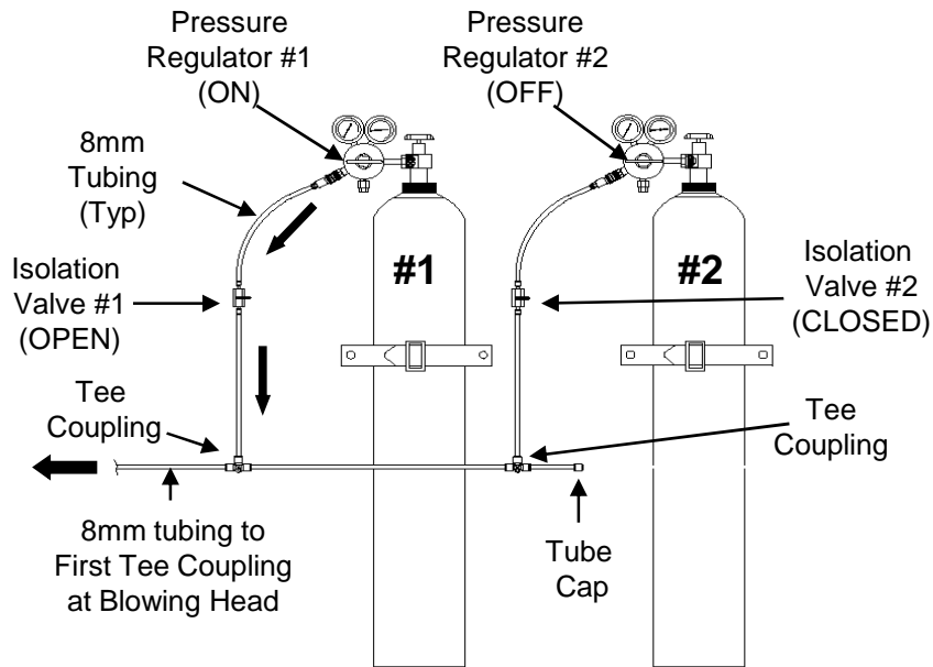
Figure 12 Dual Tank Operation; Tank #1 ON
